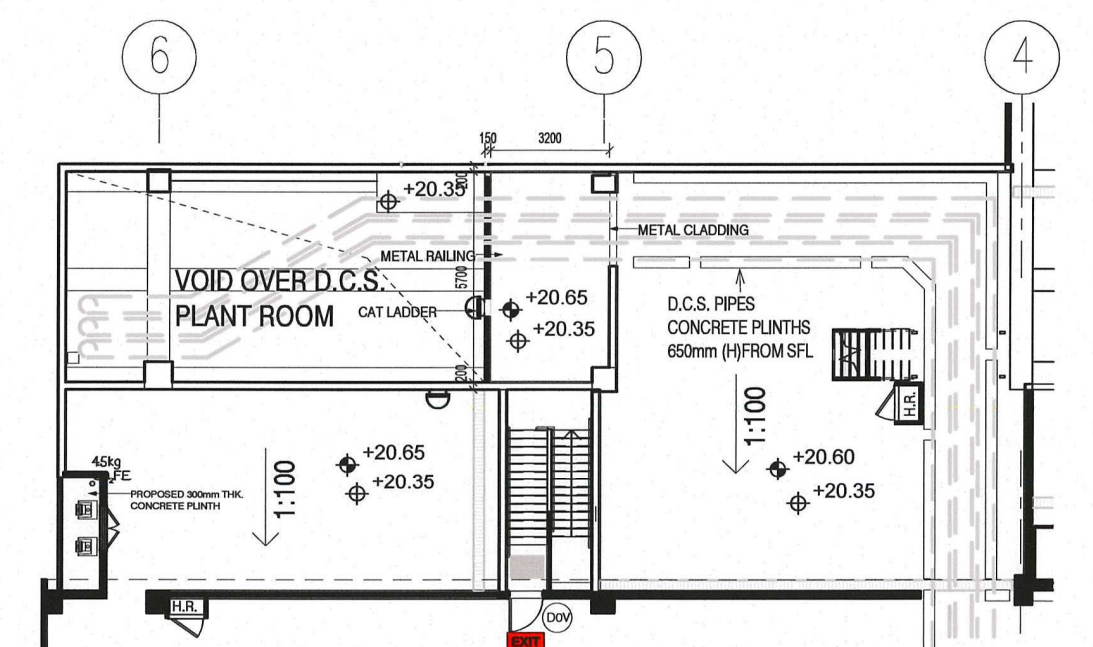
LOWER ROOF PART PLAN AT +20.35
